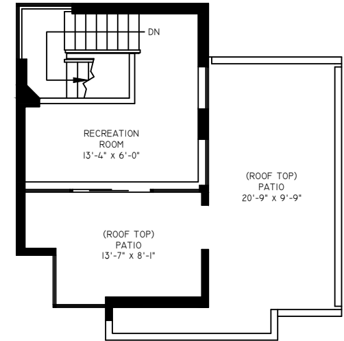
THIRD FLOOR 215 SQ. FT. 8'-0" CEILING HEIGHT
