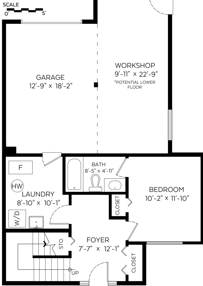
Lower Floor Plan
