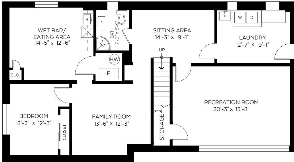
Lower Floor Plan Floor Area: 1,341 sq.ft
