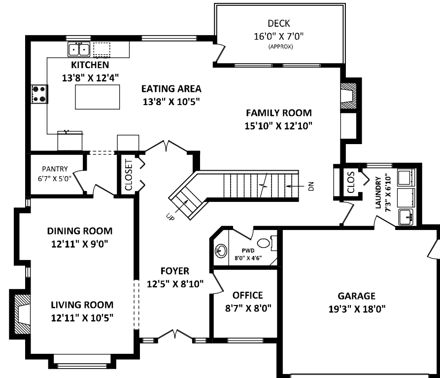
MAIN FLOOR: 1468 SQ.FT.
