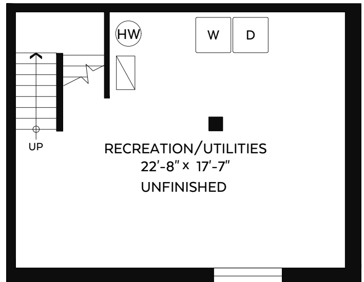
Unfinished Lower Floor Plan Floor Area: 439 sq.ft.
