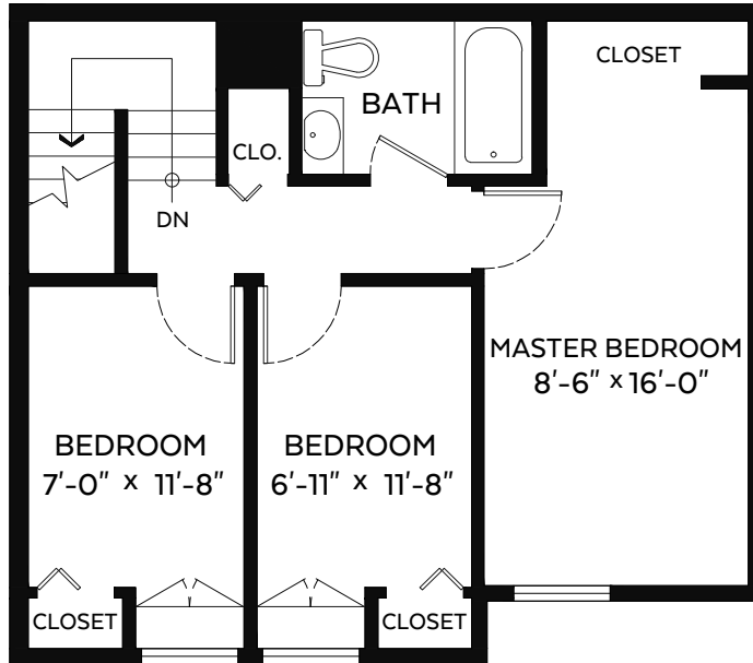
Upper Floor Plan Floor Area: 500 sq.ft.
